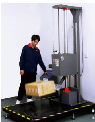
跌落测试 Drop Test
