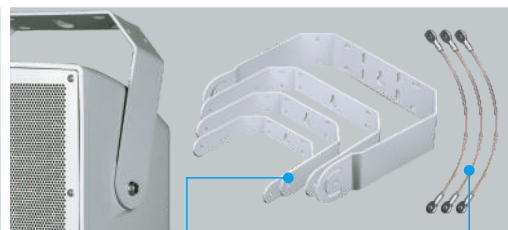
喷涂安装支架 (碳钢、不锈钢) 不锈钢保险绳 Wall bracket with powder spray (carbon steel, stainless steel), stainless steel safty rope
